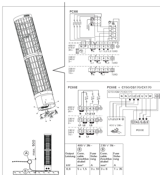
Electrical connections
